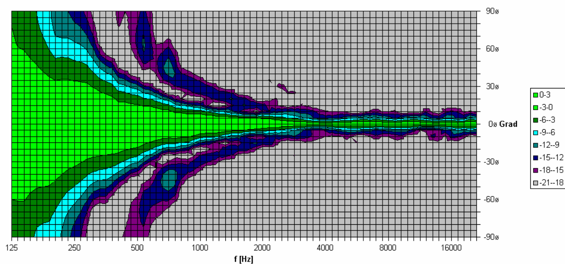
QR36 ver. Directivity Plot
