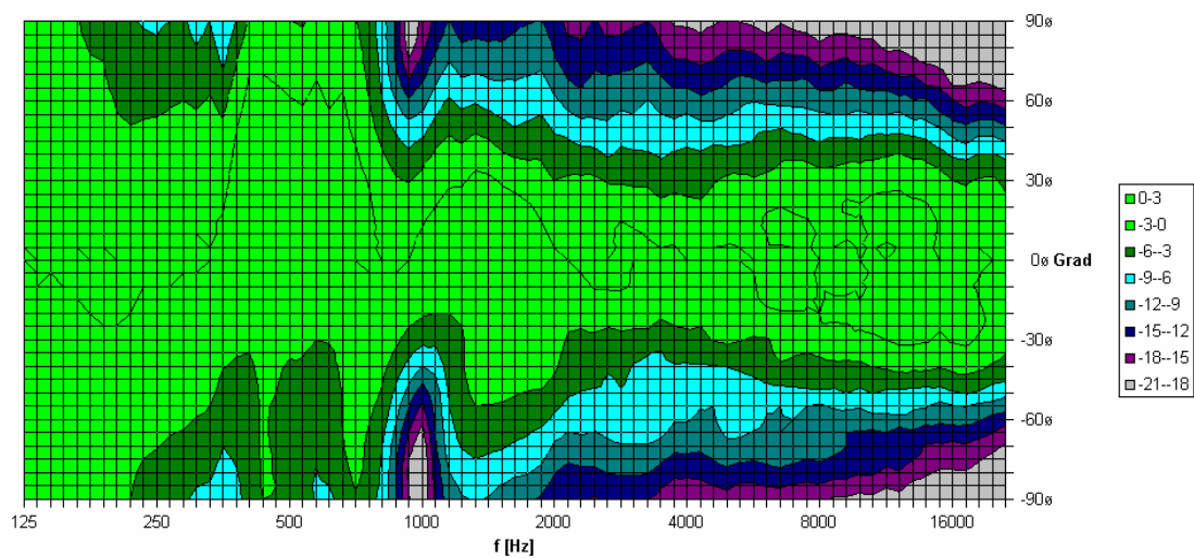
QR18 ver. Directivity Plot
